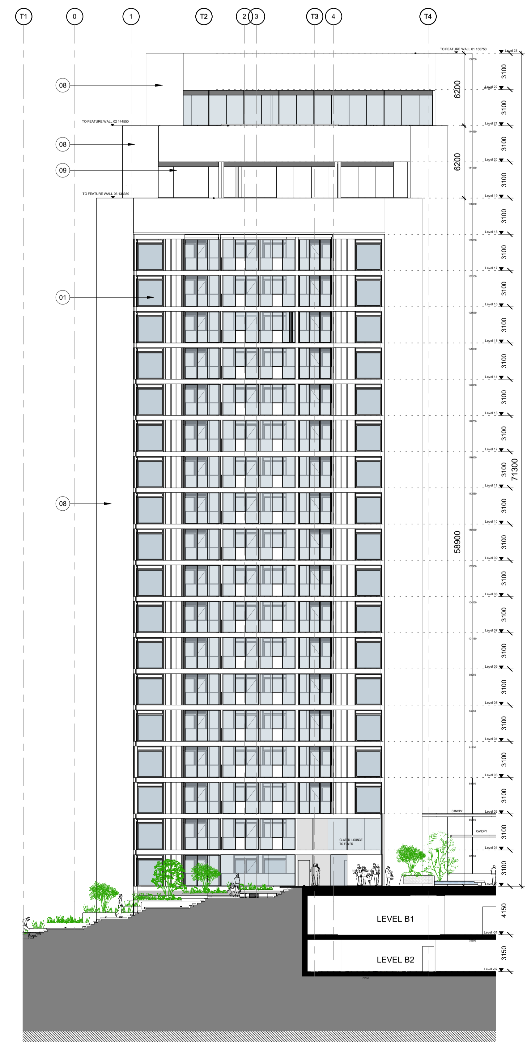
2 Block B Proposed Elevation 04 1 : 200
