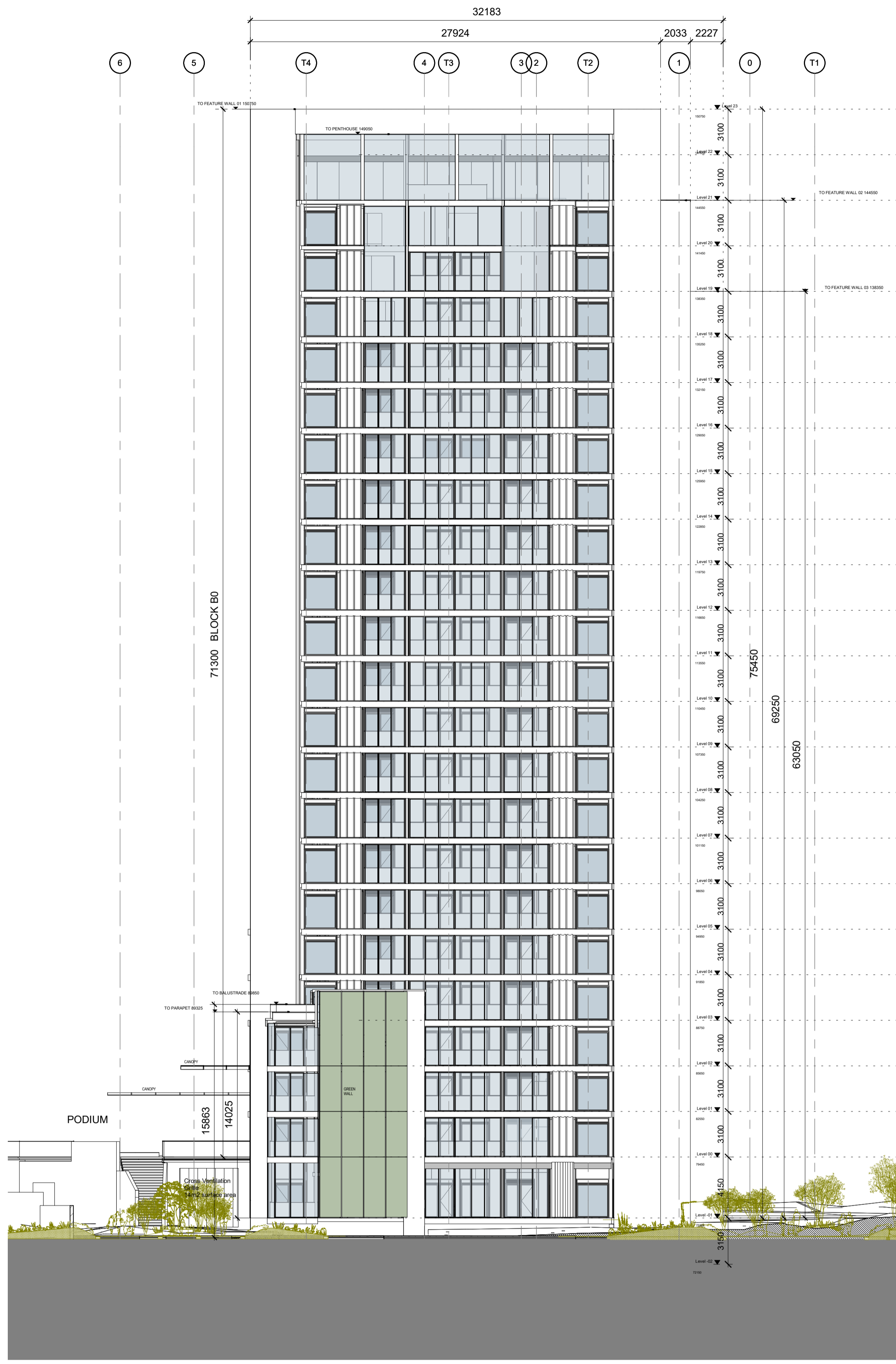
1 Block B Proposed Elevation 02 1 : 200
